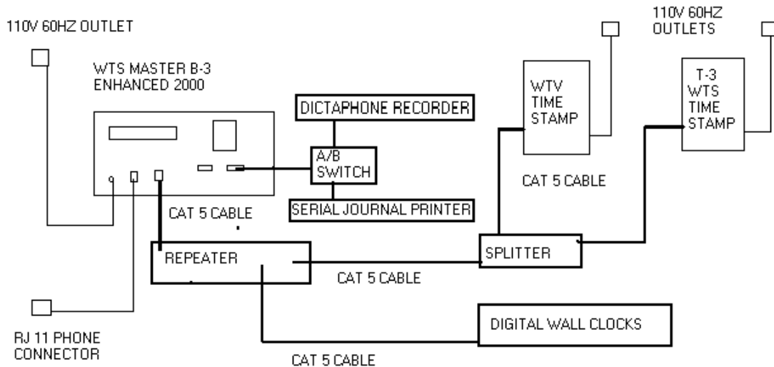
DIAGRAM OF WIDMER MASTER ATOMIC CLOCK SYSTEM B-3-911 ENHANCED
